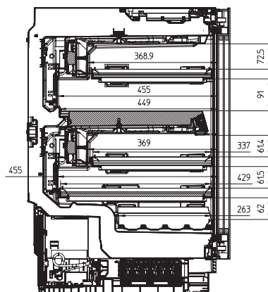
KWTUS7096E, interior dimensions (installation drawings)
