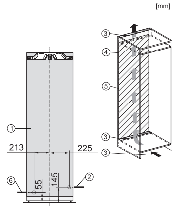
FNS7794E, FNS7774D, installation (footnote*) (installation drawings)
