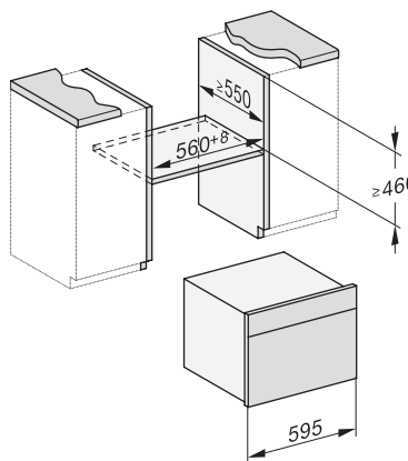
DGC7x4x, DGC7x4x installation drawings
