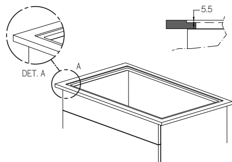
Flush top installation
